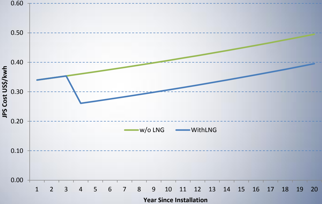
Price of JPS Power Over Time Inflated
